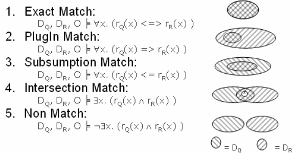
Figure 4: Set-based Matchmaking Notions
