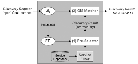
Figure 6: Service Discoverer Architecture
