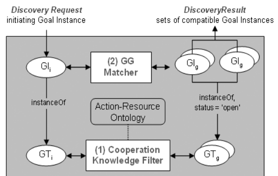
Figure 5: Partner Discoverer Architecture
